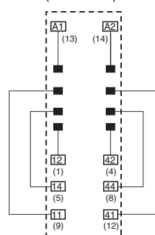
Terminal Arrangement/ Internal Connection Diagram (TOP VIEW)
