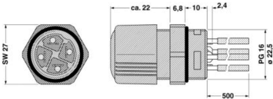
Dimensioned drawing
