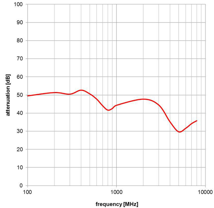
measurement based on assembled top cover with THT frame according to IEEE STD 299
