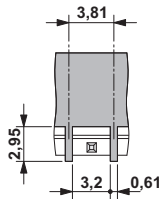
Dimensioned drawing
