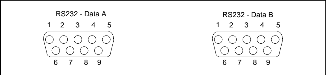
Figure 8. RS232 transmit and receive connectors: CN2, CN3
