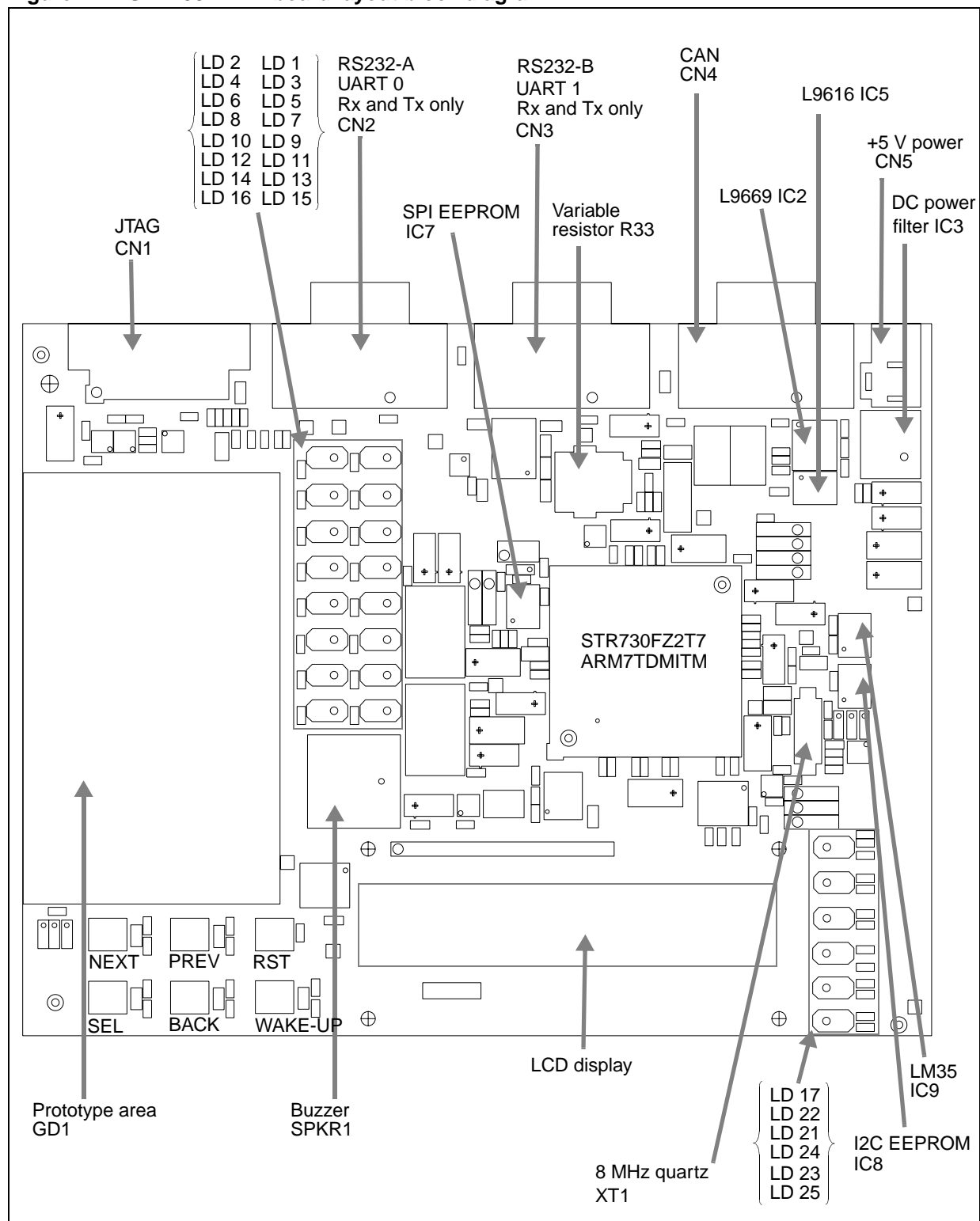
Figure 2. STR730-EVAL board layout block diagram
