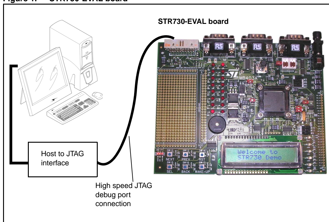
Figure 1. STR730-EVAL board
