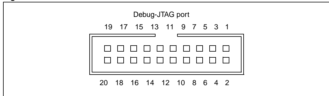
Figure 9. JTAG standard interface: CN1
