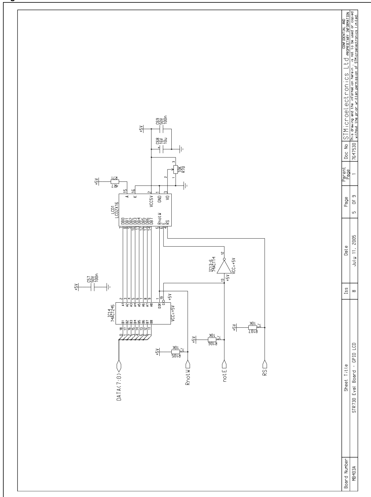
Figure 14. GPIO LCD
