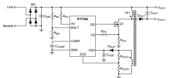
Buck-Boost Converter
