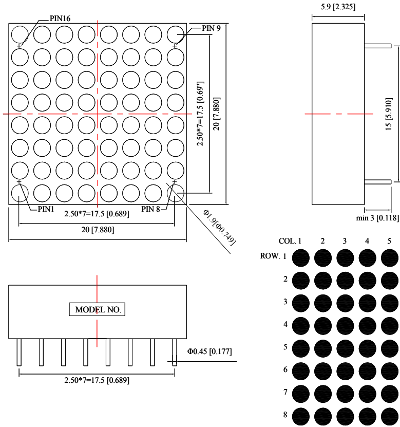
KWM-20882AUyB
