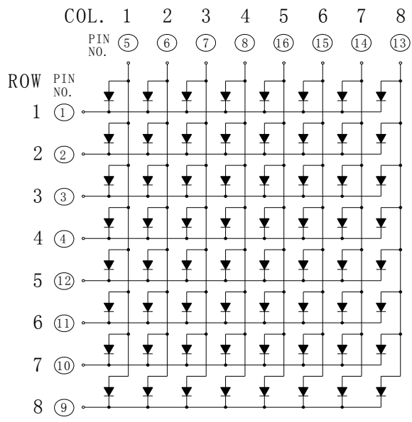
KWM-20882CUyB
