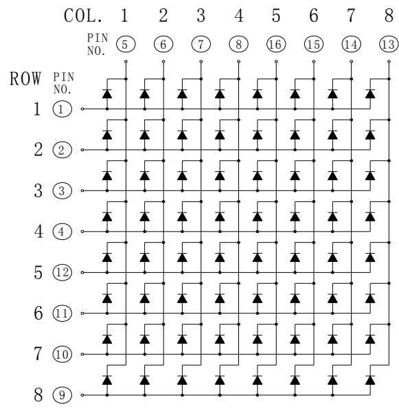
KWM-20882AUyB
