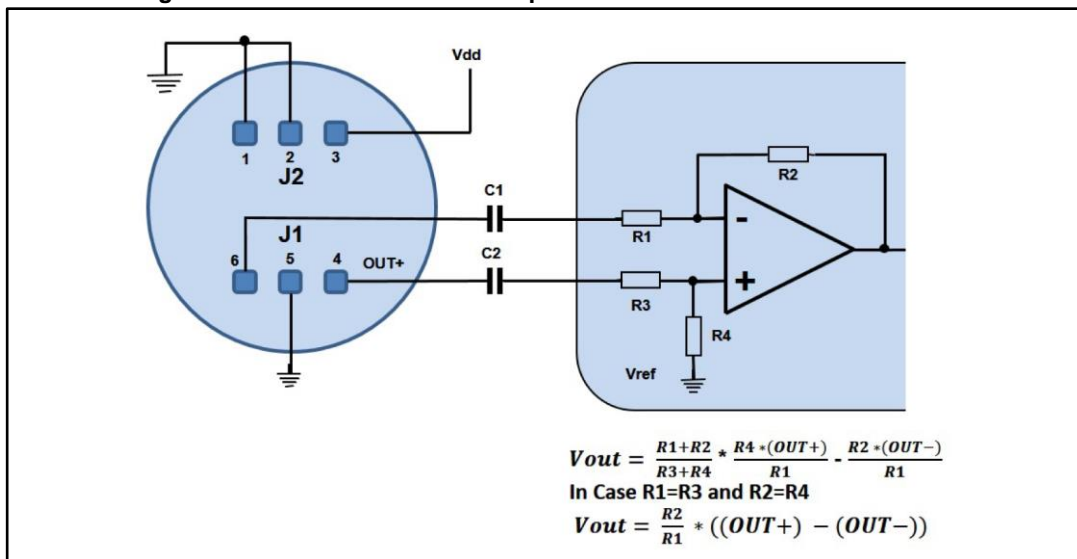
Figure 2: STEVAL-MKI139V4 example of external electrical connections
