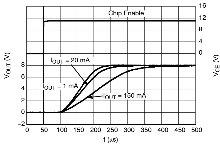
Figure 31. Start-up, 8.0 V Version, V_{IN} = 11.0 V
