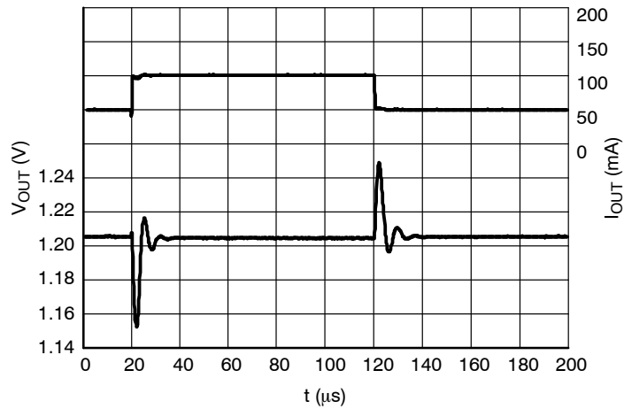
Figure 26. Load Transients, 3.0 V Version, I_{OUT} = 1 - 20 \text{ mA} , t_R = t_F = 50 \mu\text{s} , V_{IN} = 6.0 \text{ V}
