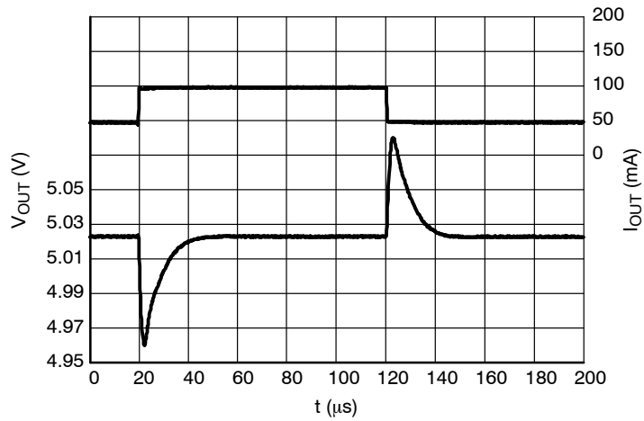
Figure 28. Load Transients, 8.0 V Version, I_{OUT} = 1 - 20 \text{ mA} , t_R = t_F = 50 \text{ } \mu\text{s} , V_{IN} = 11.0 \text{ V}
