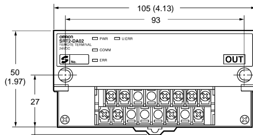
Mounting Holes
